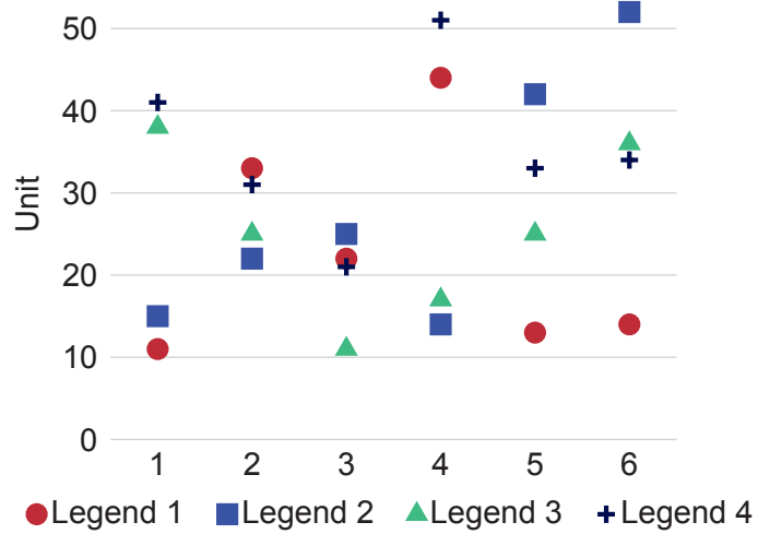
Figure 2.7: Scatter plot
