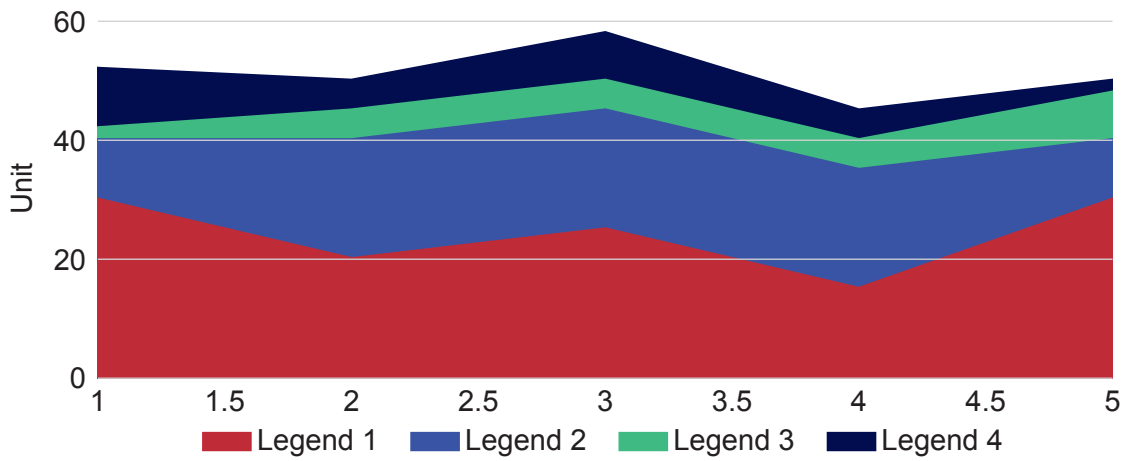
Figure 2.6: Area graph
