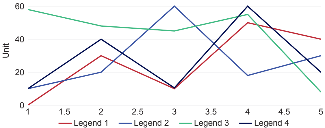
Figure 2.4: Line graph
