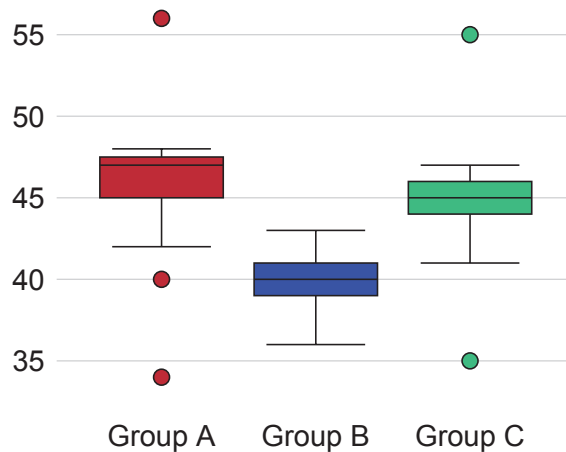
Figure 2.8: Boxplot
